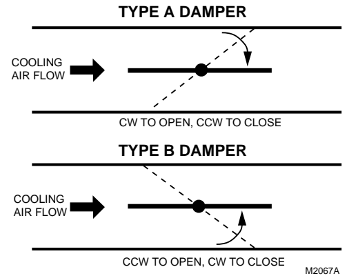
Fig. 5. Determining rotation direction (CW or CCW) for damper opening.
