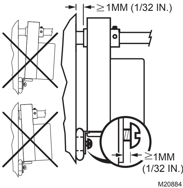
Fig. 4. Mounting W7751H to VAV box damper housing when actuator is not parallel to VAV box damper housing.
