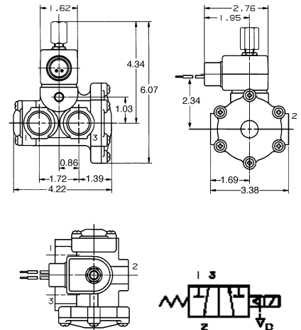
Port Identification: 1-Exhaust/ 2-Cylinder/ 3-Pressure
