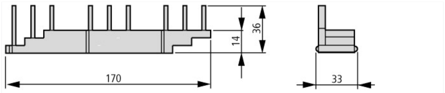
Three-phase commoning link
